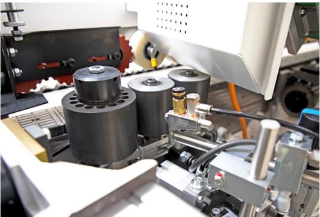
Pressure zone Heavy pressure zone up to 8 mm edge thickness and 60 mm panel height for optimum glue joint quality.
